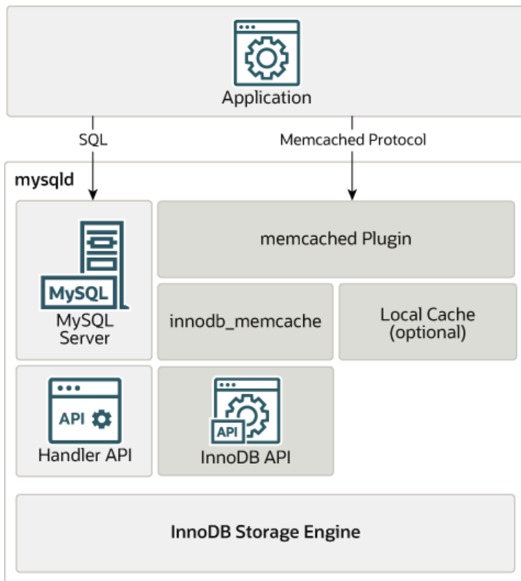
Figure 14.4 MySQL Server with Integrated memcached Server
