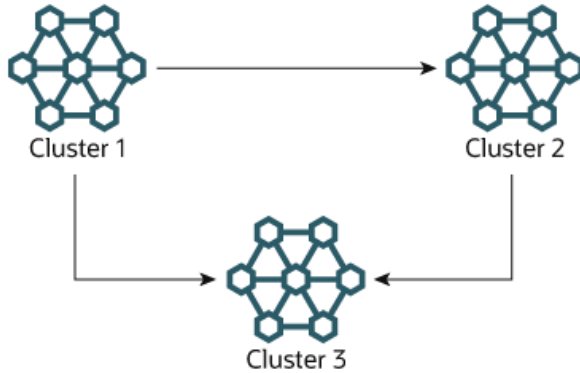
Figure 21.19 NDB Cluster Multi-Master Replication With 3 Sources
