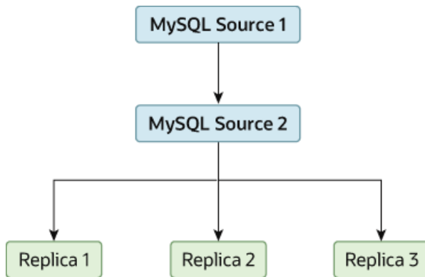
Figure 16.3 Using an Additional Replication Source to Improve Performance
