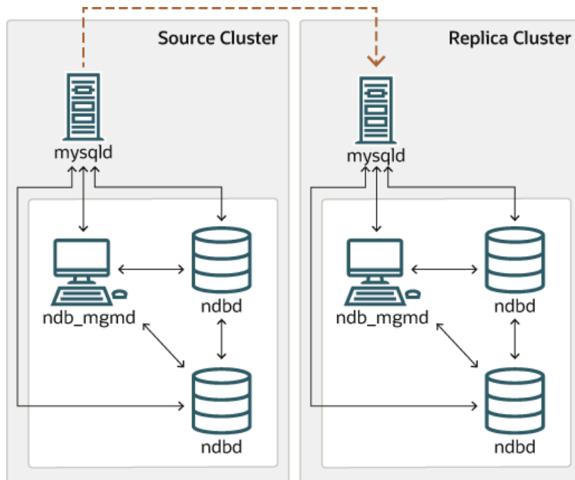
Figure 21.15 Replication Between SQL Nodes Connected Using IPv6
