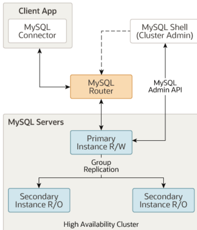
Figure 20.1 InnoDB Cluster overview
