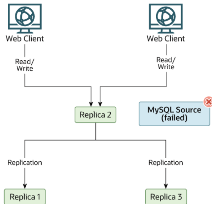
Figure 16.5 Redundancy Using Replication, After Source Failure
