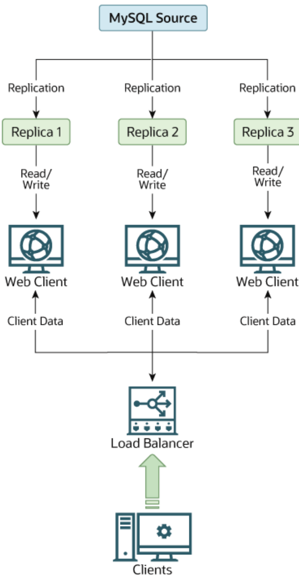
Figure 16.1 Using Replication to Improve Performance During Scale-Out
