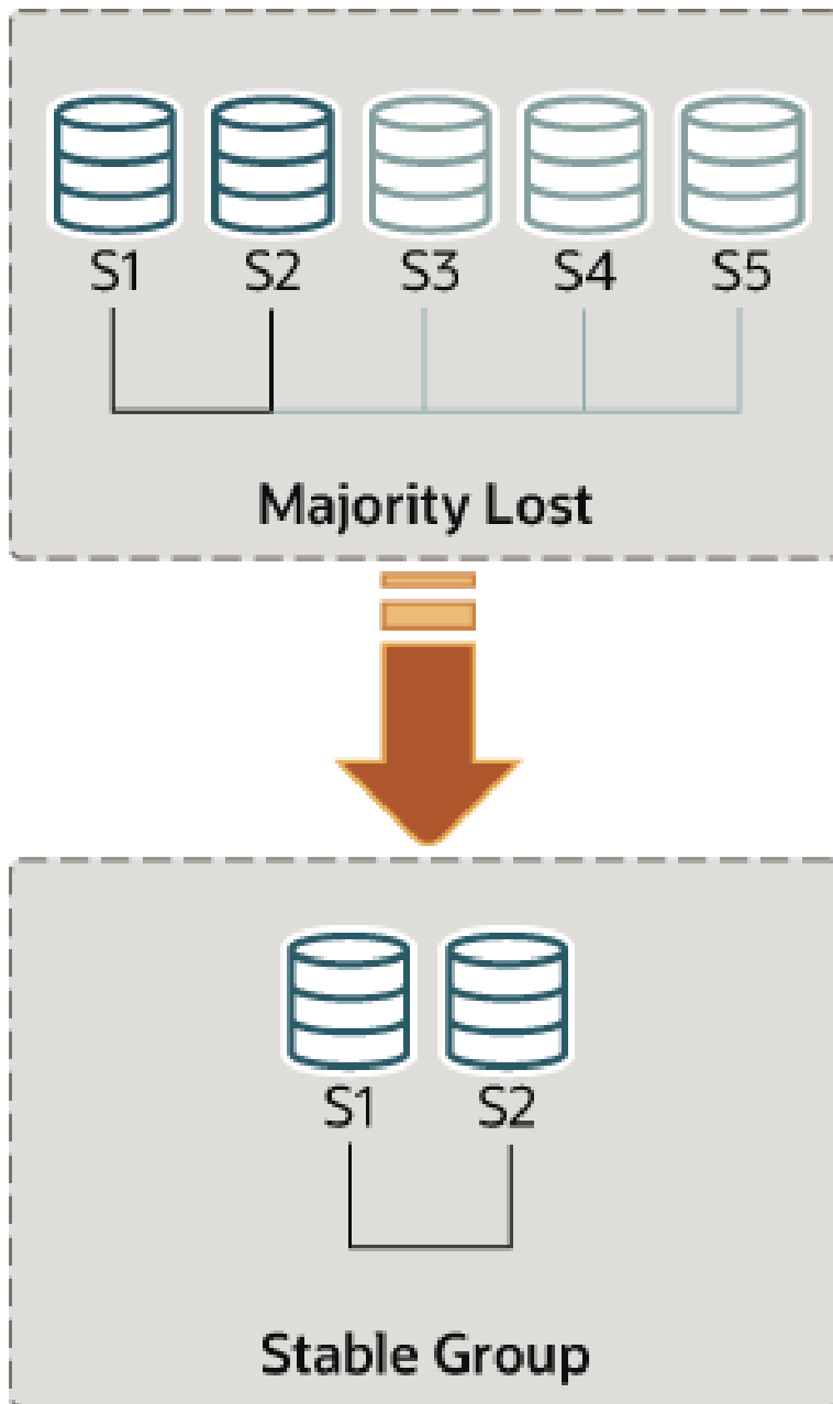
Figure 17.8 Forcing a New Membership
