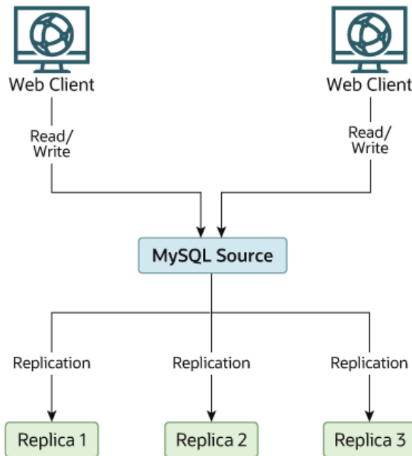
Figure 16.4 Redundancy Using Replication, Initial Structure
