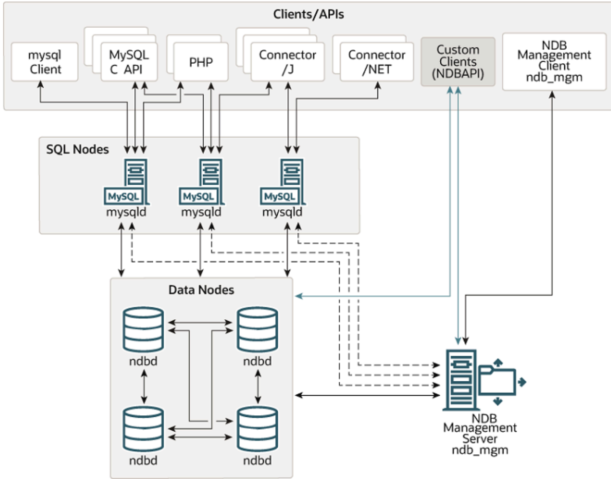
Figure 21.1 NDB Cluster Components
