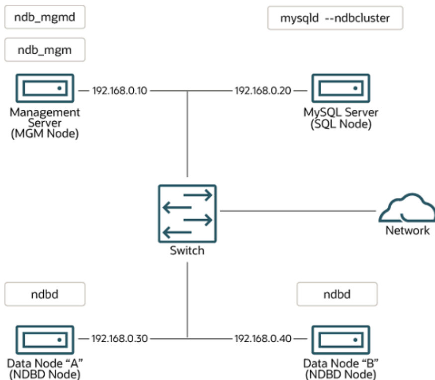
Figure 21.4 NDB Cluster Multi-Computer Setup
