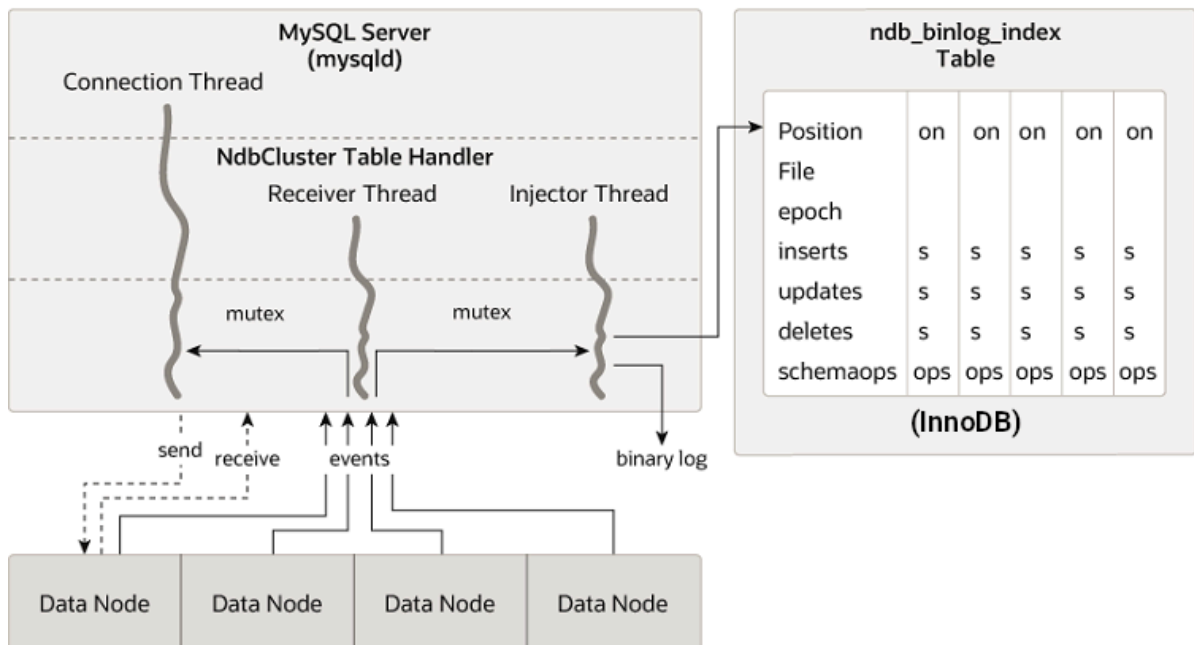
Figure 21.16 The Replication Source Cluster
